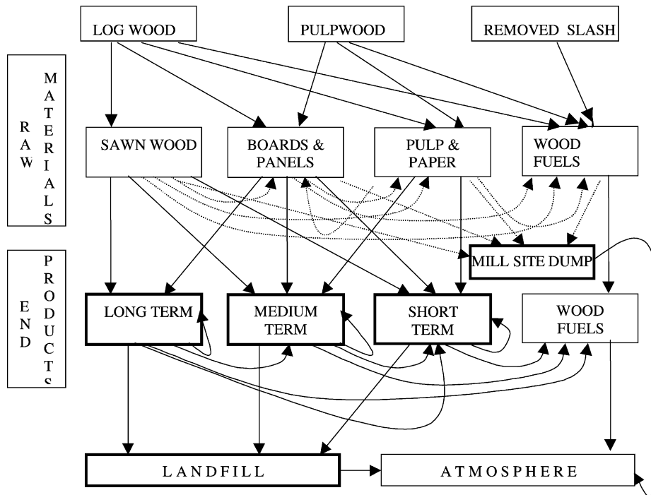
Fig. 3. Outline of the wood product module. Arrows show transfers of carbon between different phases of life span (from harvest to final allocation). Boxes with bold lines are stocks of carbon.
