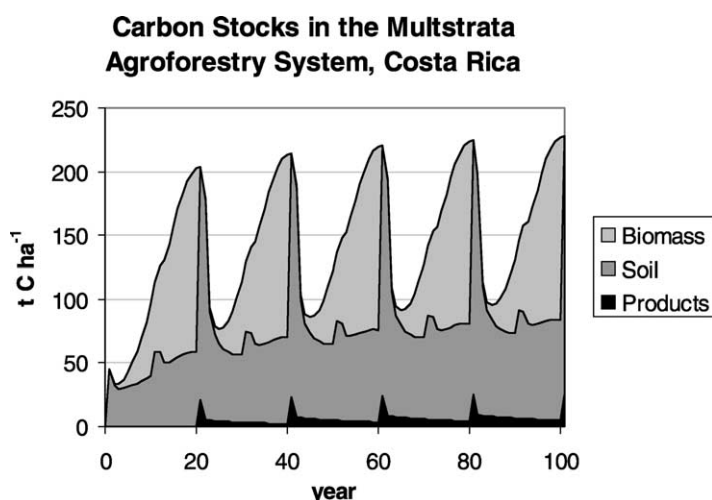
Fig. 7. Evolution of carbon stocks of a multiple cohort-agroforestry (coffee) plantation in Costa Rica.
