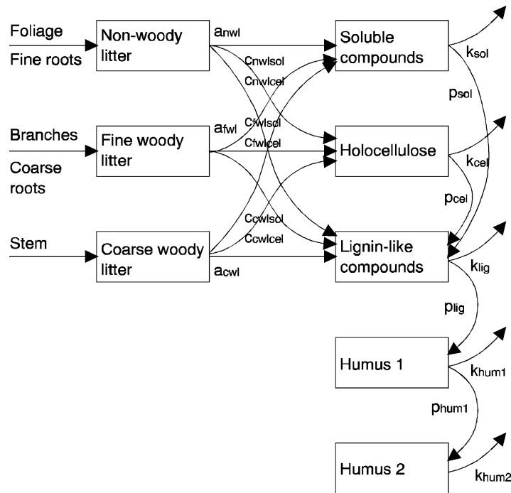
Fig. 2. Flow chart of the soil submodel. The boxes represent carbon compartments, the arrows carbon fluxes with associated acronyms of parameters controlling the fluxes.
