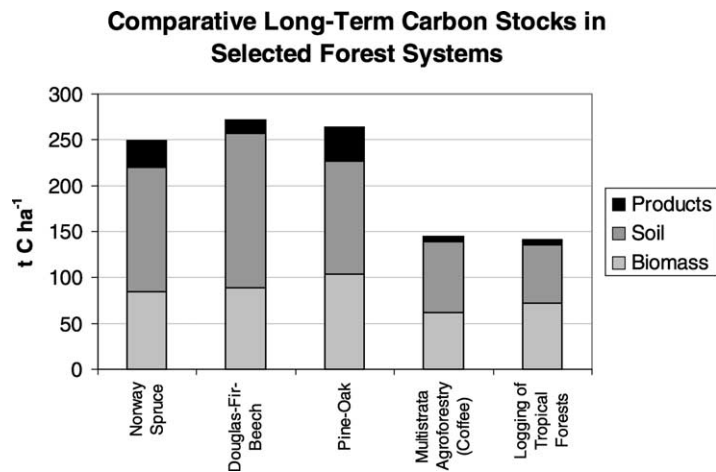
Fig. 9. Comparative long-term carbon stocks in biomass, soil, and wood products in five forestry systems.
