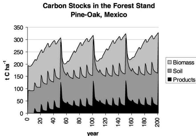
Fig. 6. Evolution of carbon stocks in an uneven-aged pine-oak native forest stand in Central Mexico.
