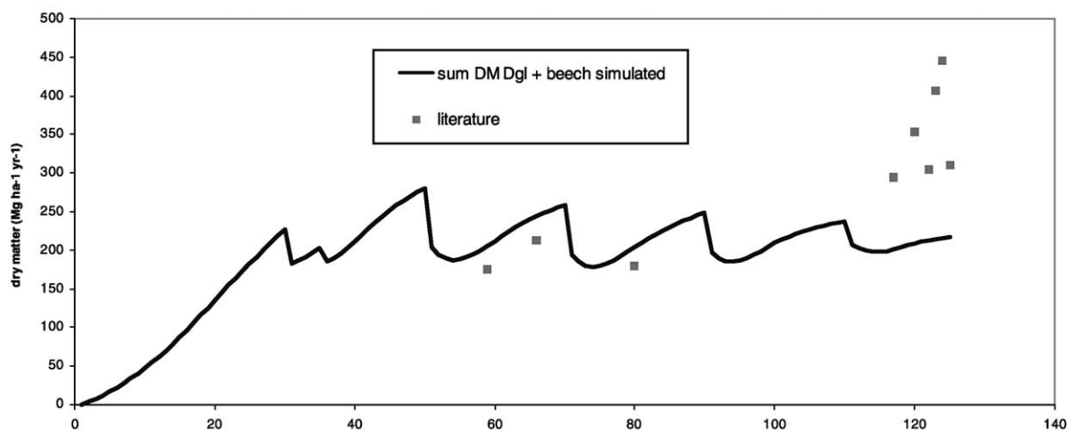
Fig. 11. Comparison of simulated dry matter stocks in the Norway spruce forest stand (top) and in the Douglas-fir-beech stand (bottom) with literature data. Sources for literature data are quoted in Nabuurs and Mohren (1993) .
