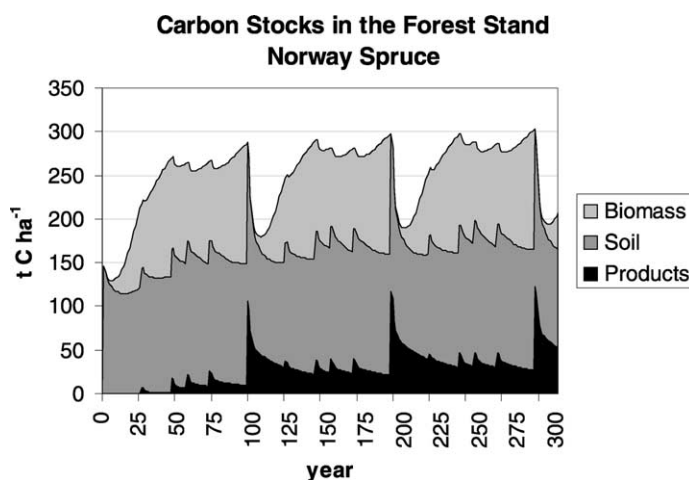
Fig. 4. Evolution of carbon stocks in a Norway spruce forest stand in Northern Europe.
