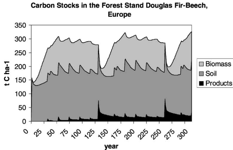
Fig. 5. Evolution of carbon stocks in an even-aged Douglas-fir-beech forest stand in Atlantic Europe.
