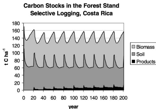
Fig. 8. Evolution of carbon stocks in a degraded tropical rainforest under selective logging in Costa Rica.
