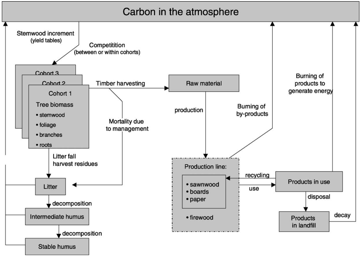
Fig. 1. Carbon fluxes/processes (arrows) and carbon stocks (boxes) in a forest ecosystem and its wood products as distinguished in CO2FIX V.2.
