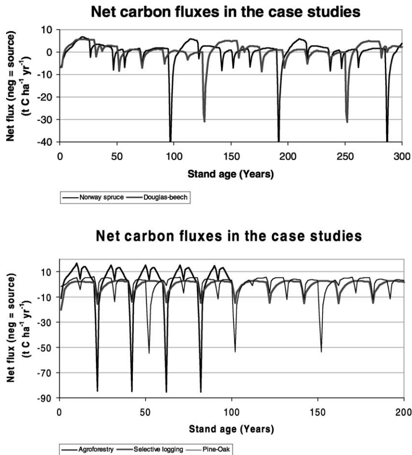
Fig. 10. Comparative net carbon fluxes in the five forestry systems selected.
