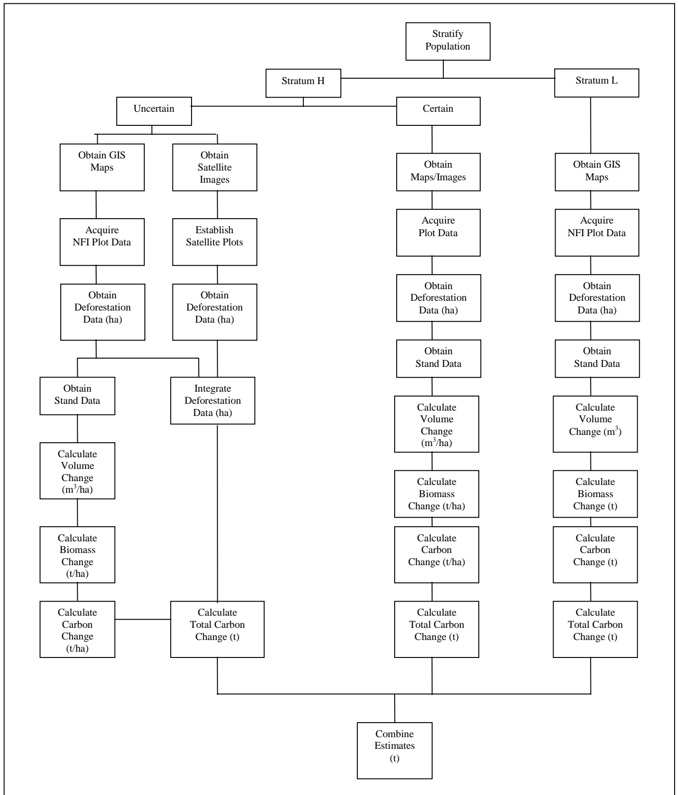
Figure 2. A schematic of the integrated, stratified core design.
