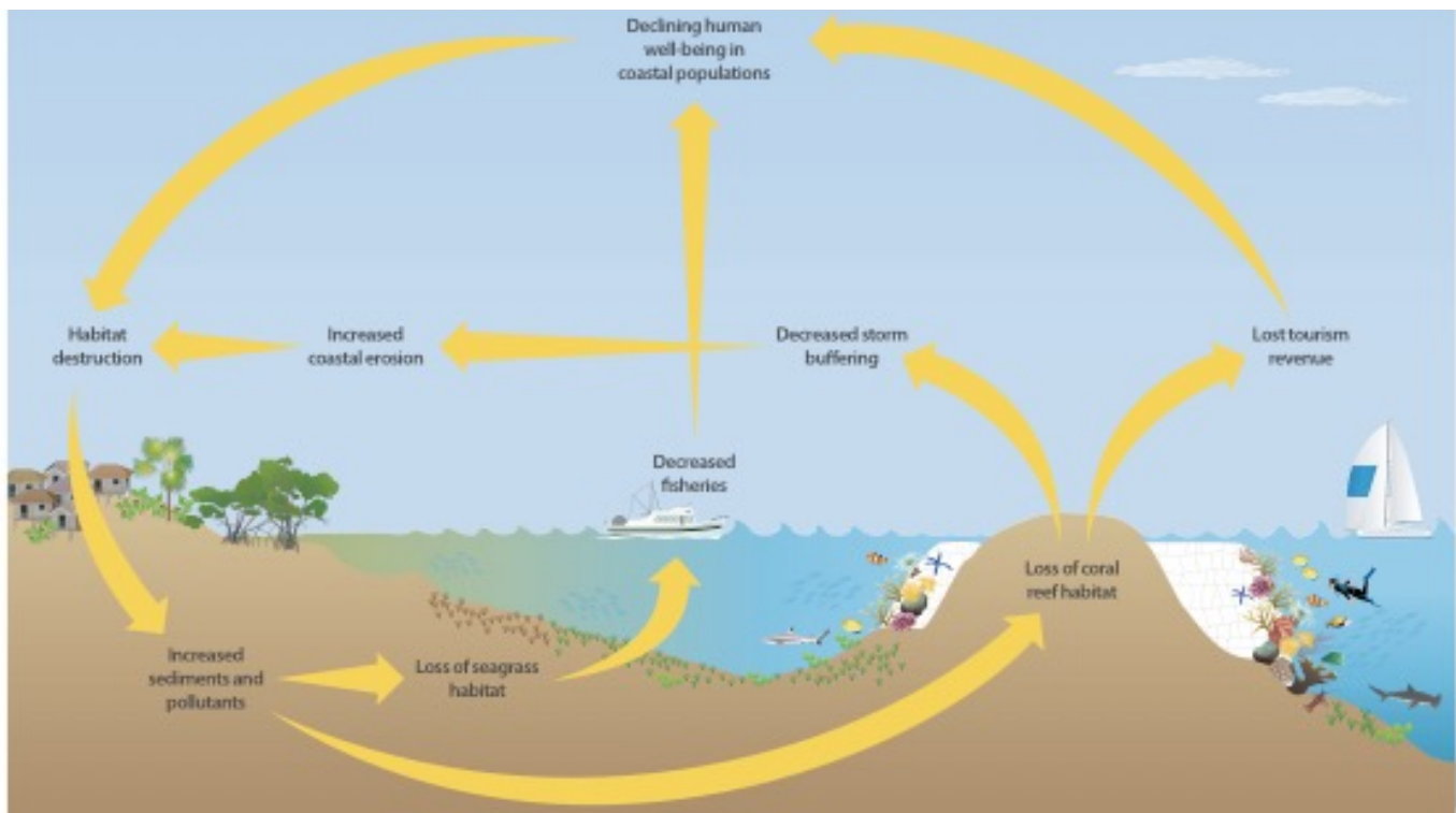
Figure 7. Connectivity and Cascading Effects of Degradation in Coastal and Marine Ecosystems
